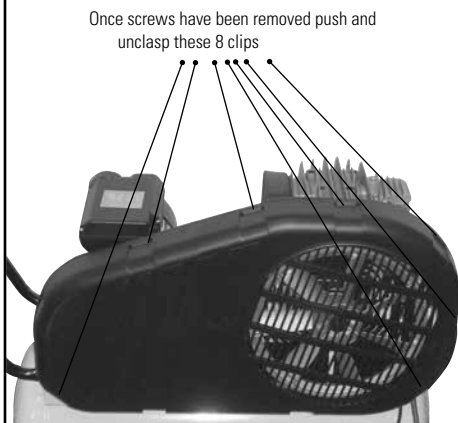
BELT GUARD SCREWS AND CLIPS
